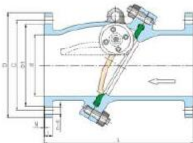
(斜盘)法兰单瓣旋启式止回阀 Flanged type tilting disc check valve
